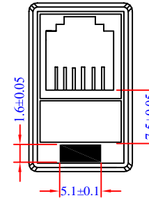
U.S 6P6C SOCKET(2)
